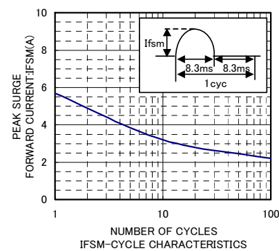
IFSM-CYCLE CHARACTERISTICS
